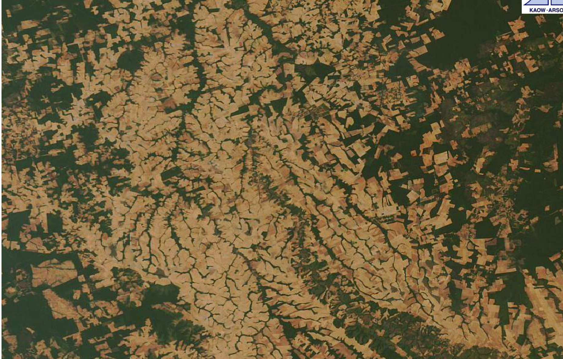
Soya bean agriculture –biofuels-feedstock-tropical deforestation-Matto Grosso. Meris August 22.08
