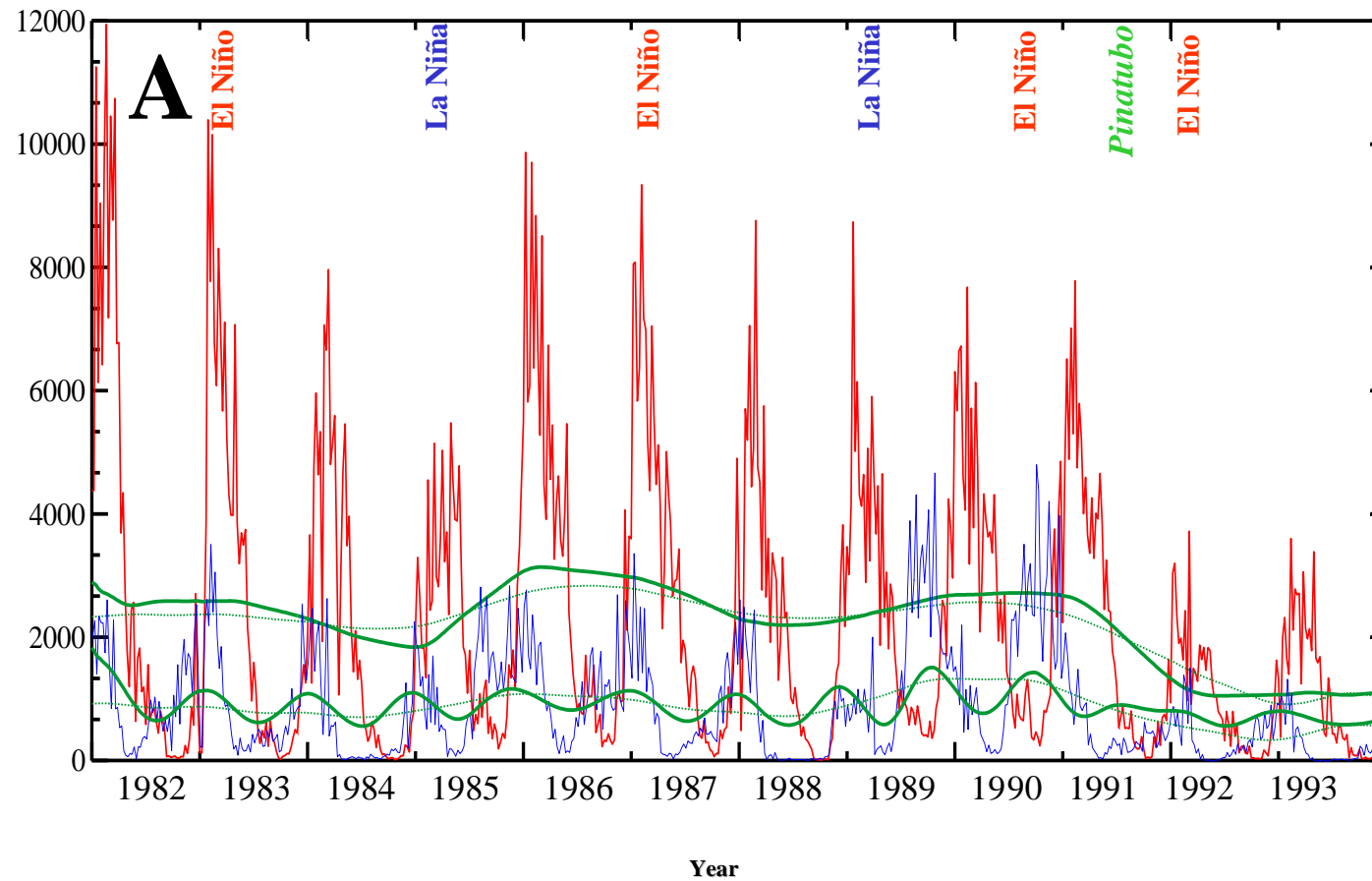
1982-93 Evolution of burned area ('000 ha) from SPOT VGT data – red:Nrth hemisphere, blue: sth hem.
